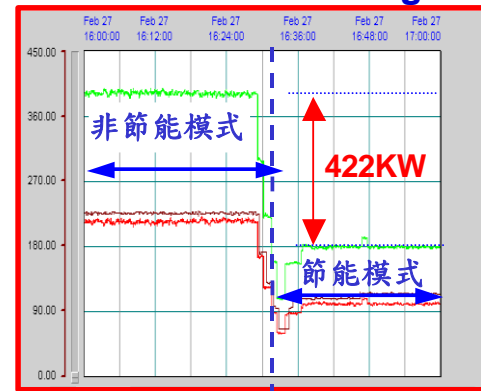
節能 422KW (65.2%)
