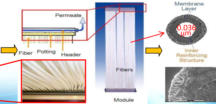
膜生物反應器 MBR(Membrane Bio-reactor)
